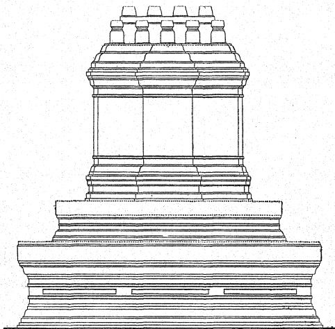
Reconstruction of the west side of the temple Si Pamoetoeng. Formerly the top was crowned by a large stupa. See p. 92.
