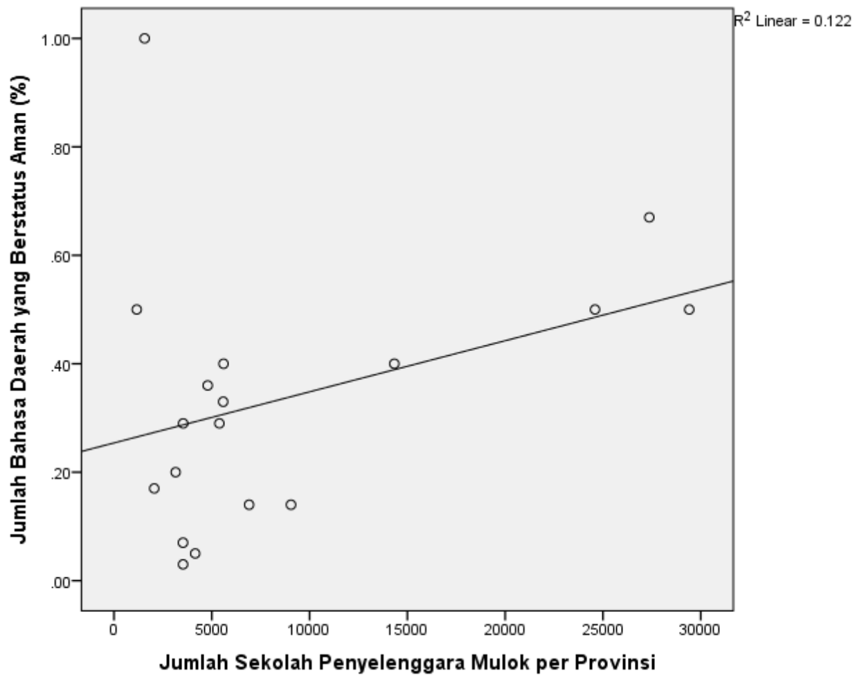
Gambar 4. 21. Diagram hasil scatter plot
